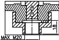
BUSHING
