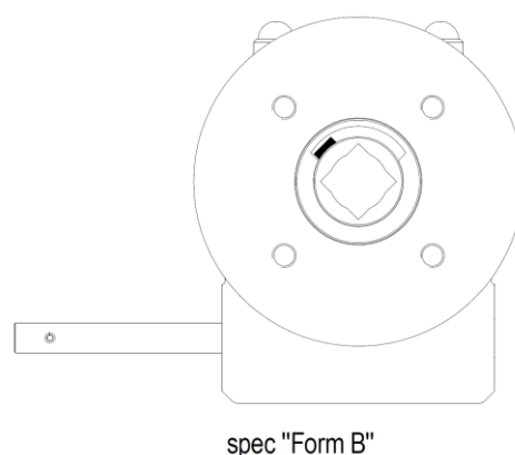
Figure 6: Position of driveshaft optional form B used for couplings for maximum stem acceptance
