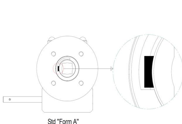
Figure 5: Standard position of driveshaft form A
