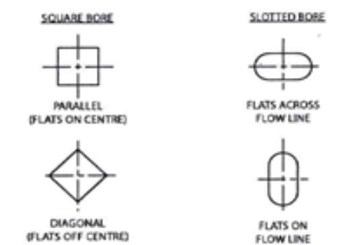
Figure 1. Drive options
