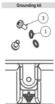
Grounding kit
