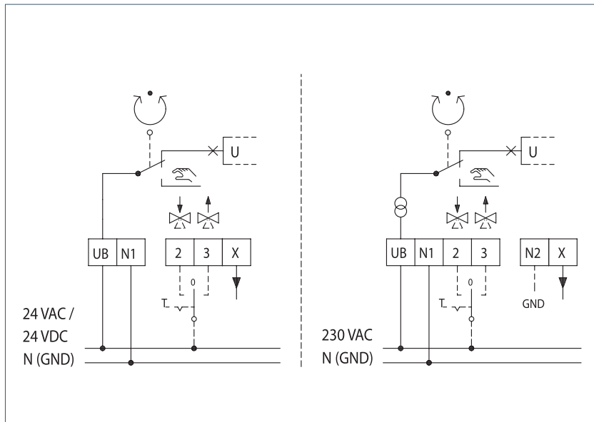
ELC 55 wiring diagram
