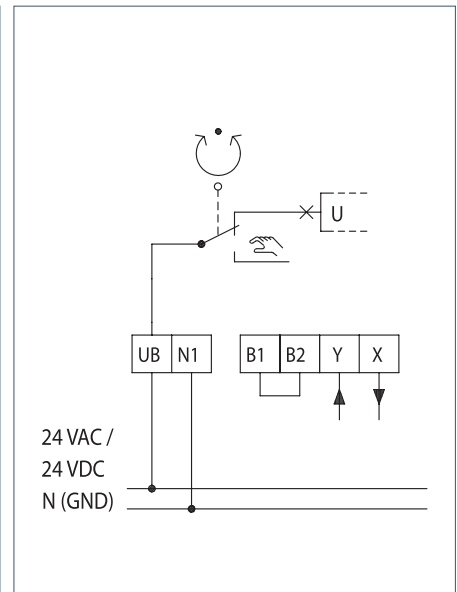
ELC 55Y wiring diagram
