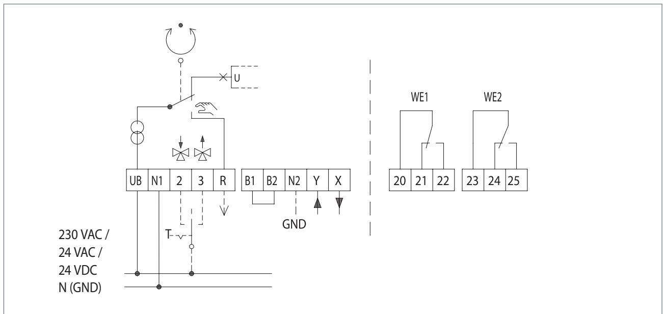
ELC 100 - 220 Wiring diagram
