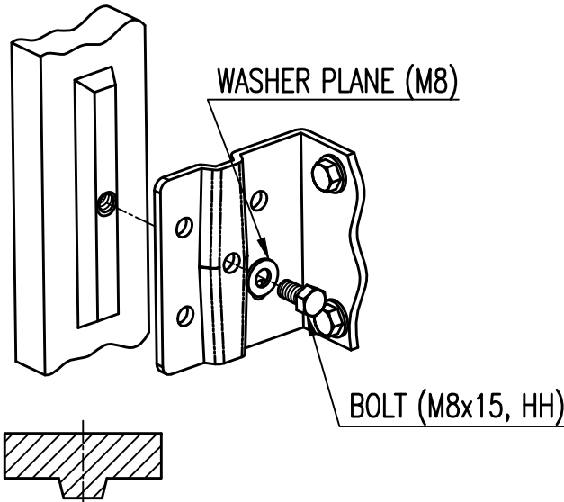
RIB TYPE ACTUATOR YOKE
