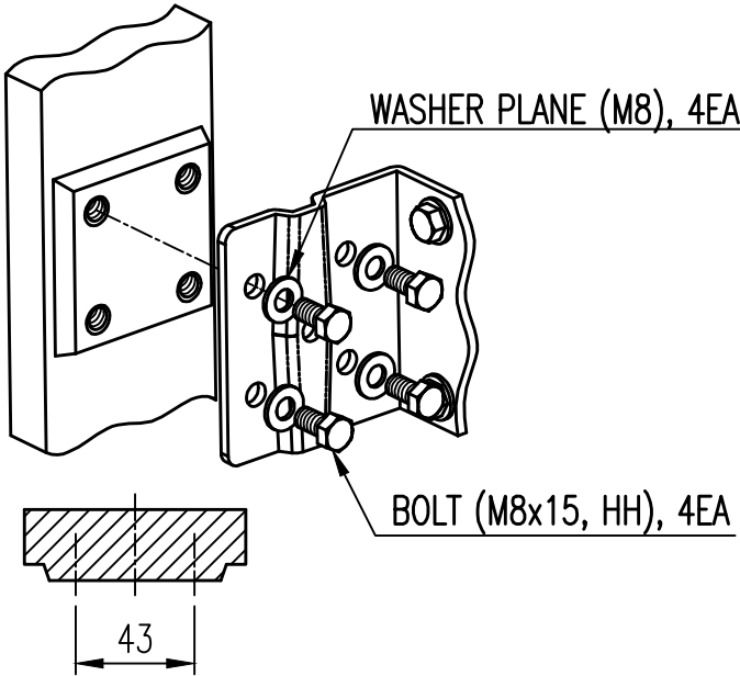
PLANE TYPE ACTUATOR YOKE
