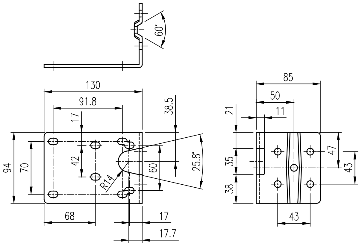
LINEAR NAMUR BRACKET (YT-1200L)
