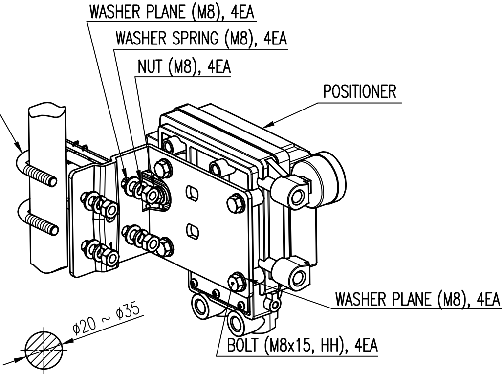
POLE TYPE ACTUATOR YOKE
